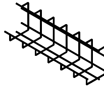
Single Tier Cable Tray H : 95mm W : 953 / 1153 / 1553mm D : 74mm
